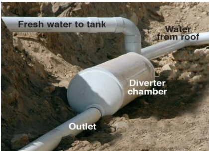
In-ground Diverter
